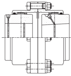
INTERFERENCE FIT
