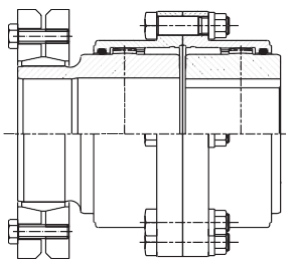
EXTERNAL CLAMPING
